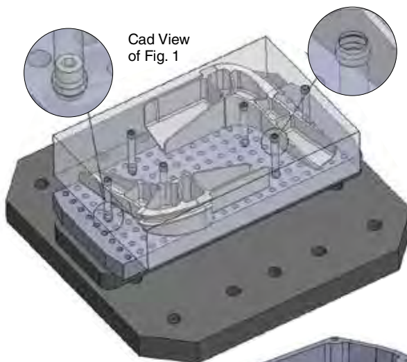
Heavy Wall Loc-Down® Bushing Part No. 11520
