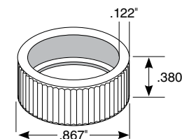
Heavy Wall Loc-Down® Bushing Part No. 11520
